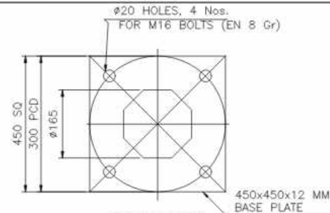
BASE PLATE
