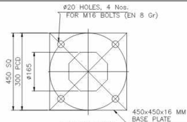
BASE PLATE
