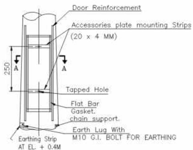
DETAIL 'Y'
