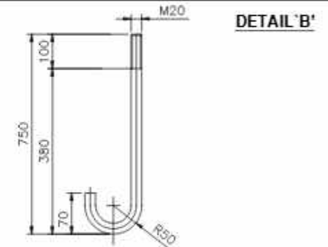
ANCHOR BOLT DETAIL (TOTAL LENGTH-750 mm)
