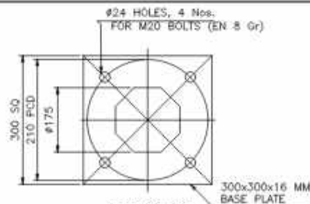
BASE PLATE
