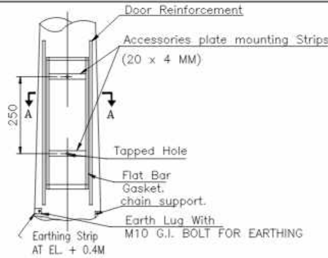
DETAIL 'Y'
