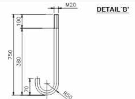
ANCHOR BOLT DETAIL (TOTAL LENGTH-750 mm)
