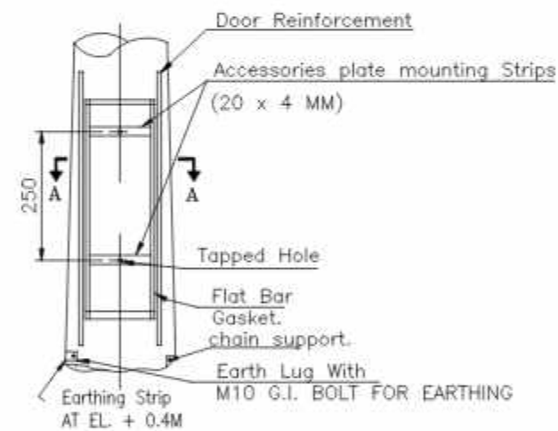
DETAIL 'Y'
