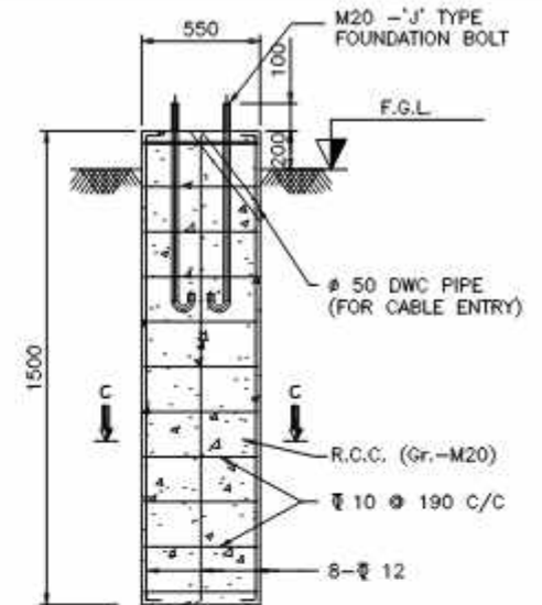
DETAIL OF CIVIL FOUNDATION
