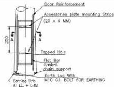
DETAIL 'Y'
