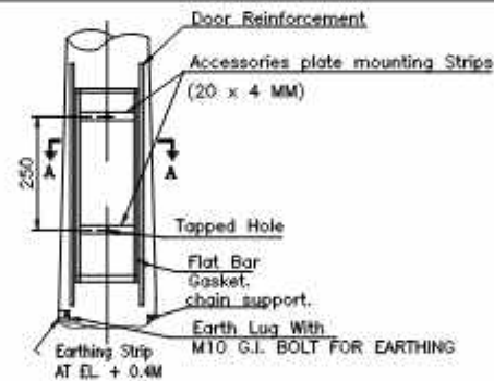
DETAIL 'Y'
