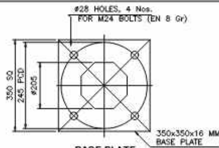
BASE PLATE
