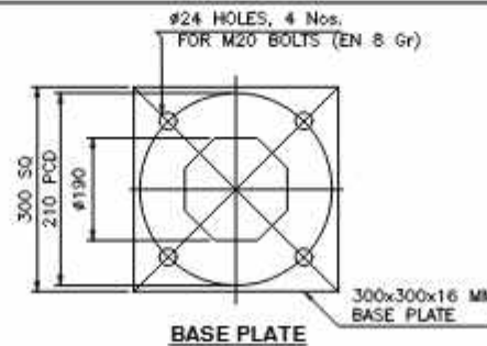
BASE PLATE
