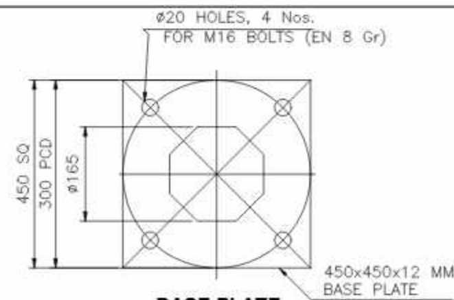
BASE PLATE
