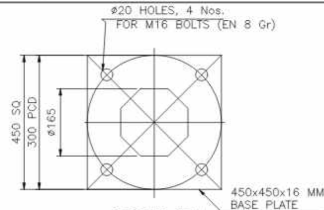
BASE PLATE
