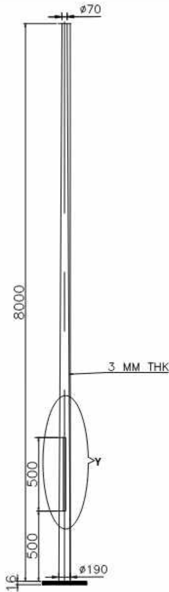
GA. DWG. OF 8 MTR. HEIGHT STANDARD CONICAL POLE
