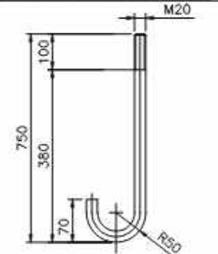
ANCHOR BOLT DETAIL (TOTAL LENGTH-750 mm)
