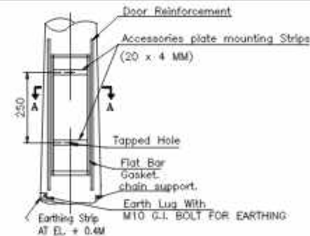
DETAIL 'Y'
