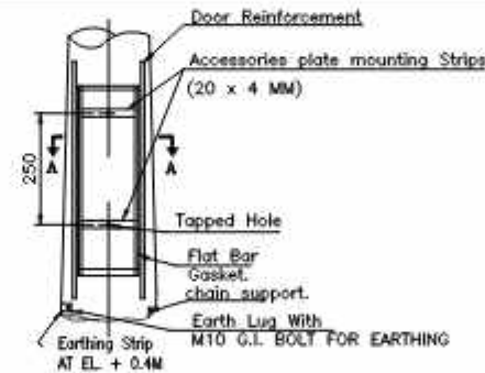
DETAIL 'Y'
