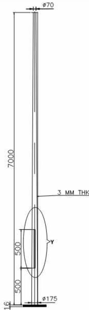
GA DWG. OF 7 MTR. HEIGHT STANDARD CONICAL POLE
