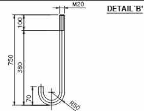
ANCHOR BOLT DETAIL (TOTAL LENGTH-750 mm)
