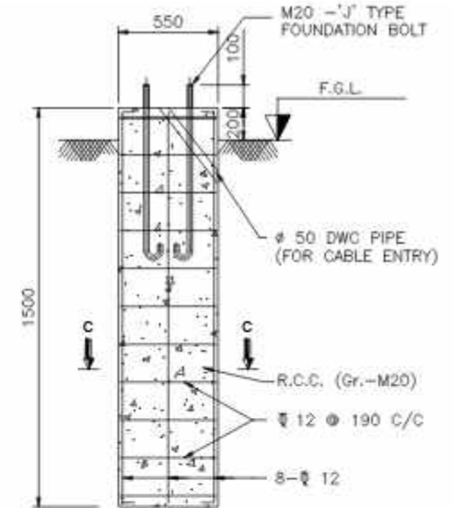
DETAIL OF CIVIL FOUNDATION
