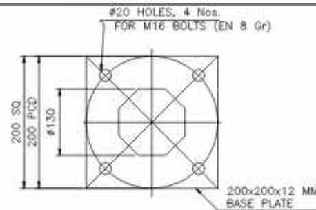
BASE PLATE
