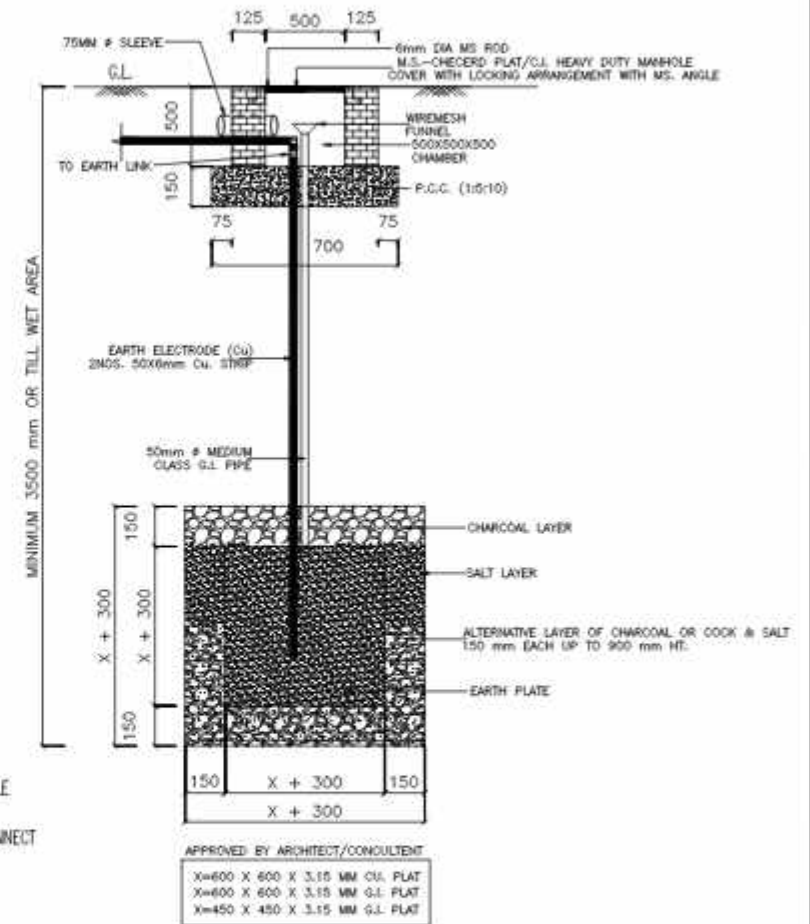
TYPICAL PLATE TYPE EARTHING DETAIL
