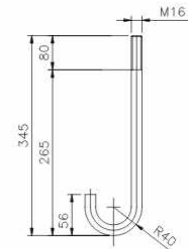
ANCHOR BOLT DETAIL (TOTAL LENGTH-450 mm)
