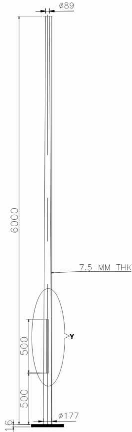
GA. DWG. OF 6 MTR. HEIGHT STANDARD FRP POLE
