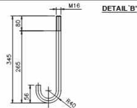
ANCHOR BOLT DETAIL (TOTAL LENGTH-345 mm)
