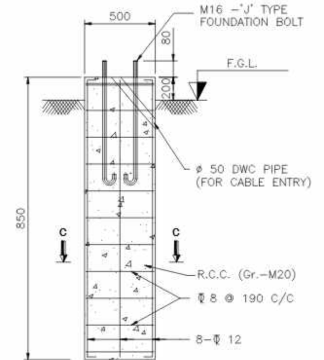
DETAIL OF CIVIL FOUNDATION
