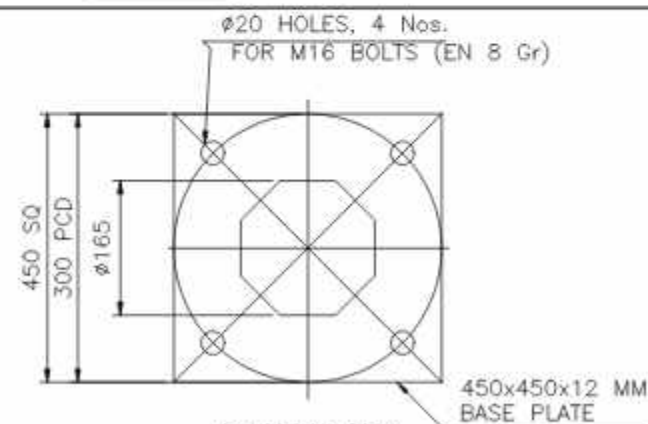
BASE PLATE
