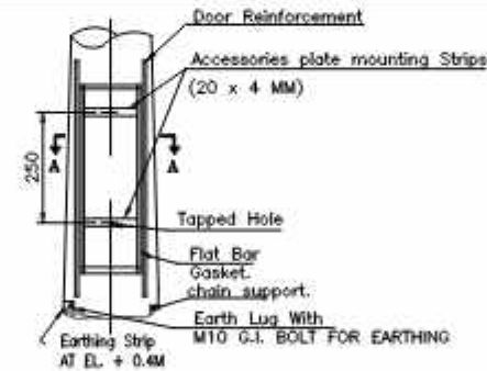
DETAIL 'Y'
