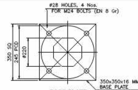
BASE PLATE
