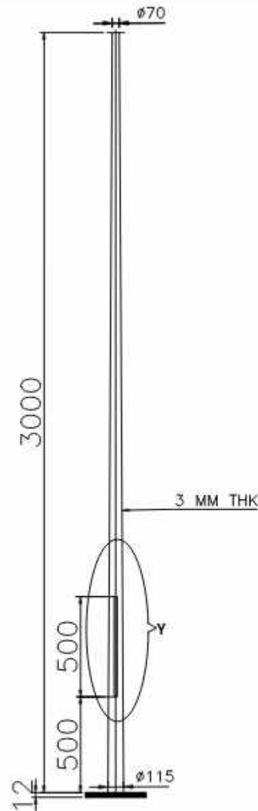
GA. DWG. OF 3 MTR. HEIGHT STANDARD CONICAL POLE
