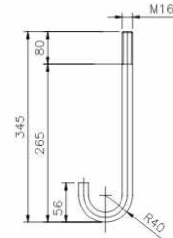
ANCHOR BOLT DETAIL (TOTAL LENGTH-345 mm)
