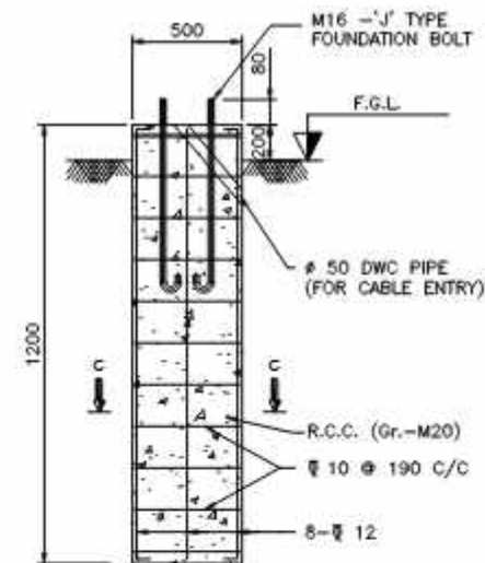
DETAIL OF CIVIL FOUNDATION
