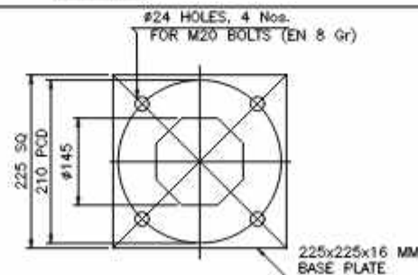
BASE PLATE
