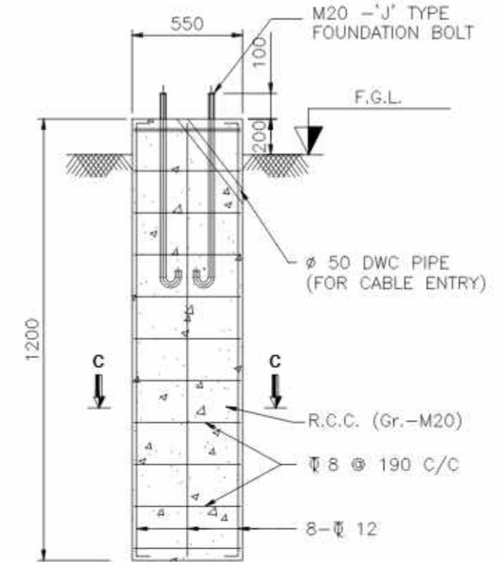
DETAIL OF CIVIL FOUNDATION
