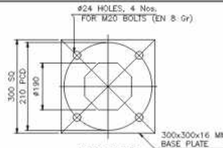
BASE PLATE
