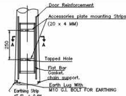
DETAIL 'Y'
