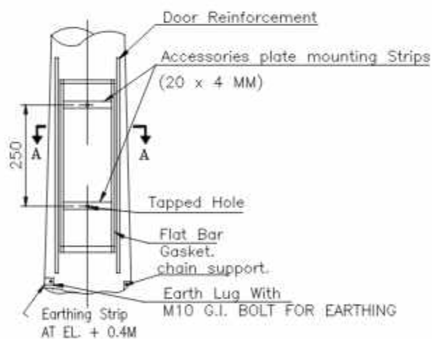
DETAIL 'Y'
