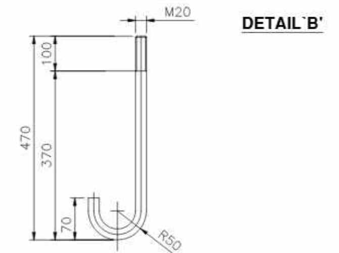
ANCHOR BOLT DETAIL (TOTAL LENGTH-470 mm)
