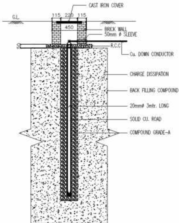
TYPICAL DETAIL FOR CHEMICAL EARTHING
