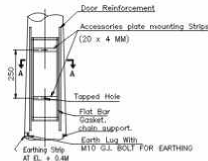
DETAIL 'Y'
