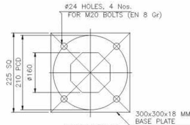
BASE PLATE
