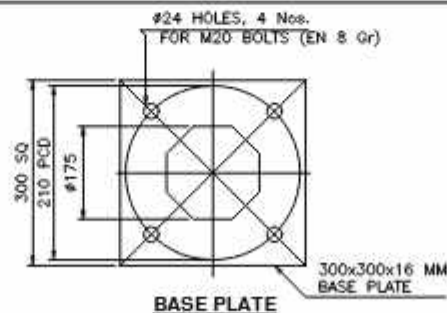
BASE PLATE
