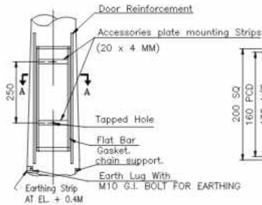
DETAIL 'Y'
