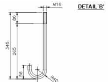
ANCHOR BOLT DETAIL (TOTAL LENGTH=345 mm)
