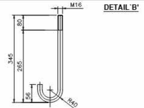
ANCHOR BOLT DETAIL (TOTAL LENGTH-345 mm)
