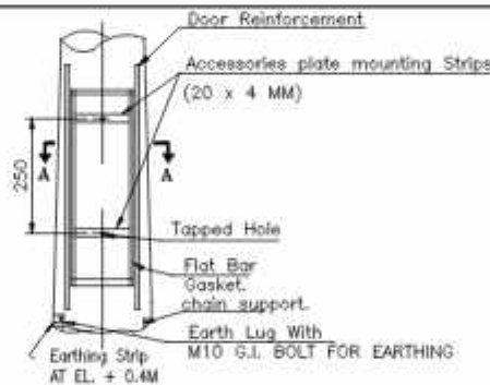
DETAIL 'Y'
