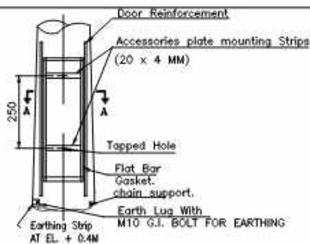
DETAIL 'Y'
