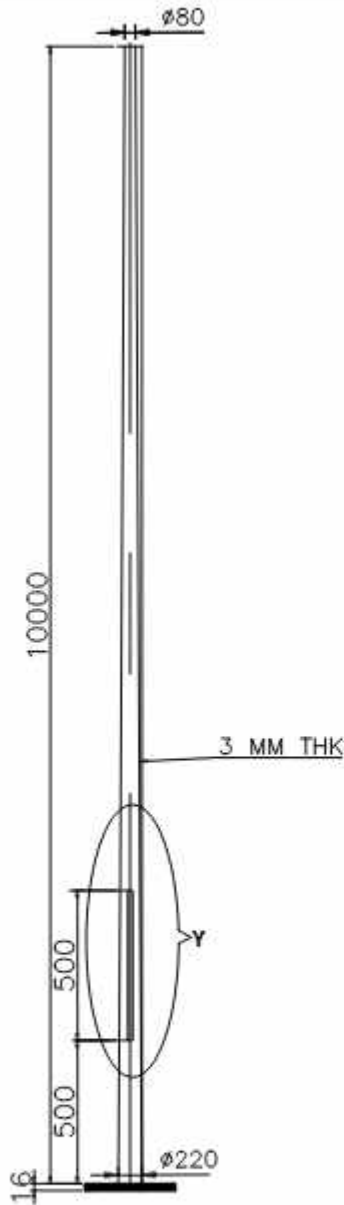
GA. DWG. OF 10 MTR. HEIGHT STANDARD CONICAL POLE
