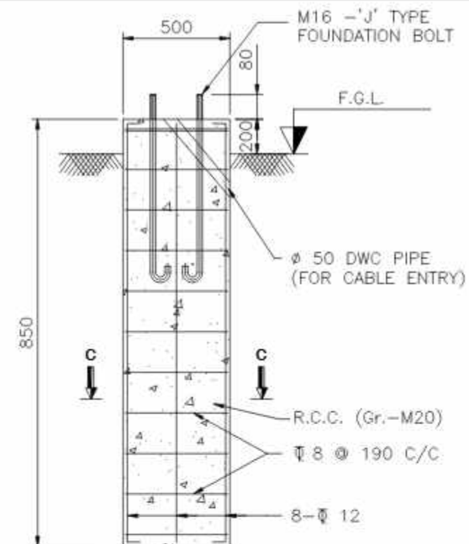
DETAIL OF CIVIL FOUNDATION
