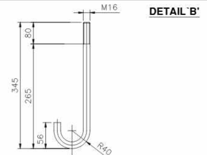
ANCHOR BOLT DETAIL (TOTAL LENGTH-450 mm)
