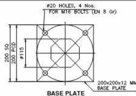
BASE PLATE
