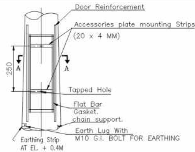
DETAIL 'Y'
