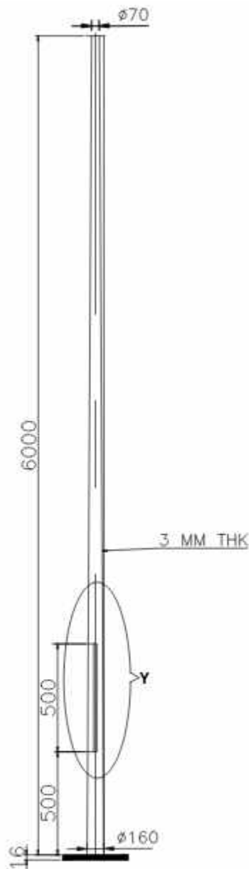
GA. DWG. OF 6 MTR. HEIGHT STANDARD CONICAL POLE
