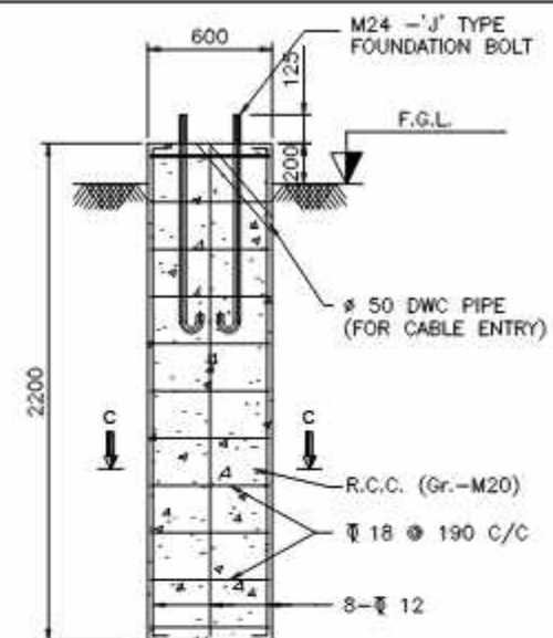
DETAIL OF CIVIL FOUNDATION
