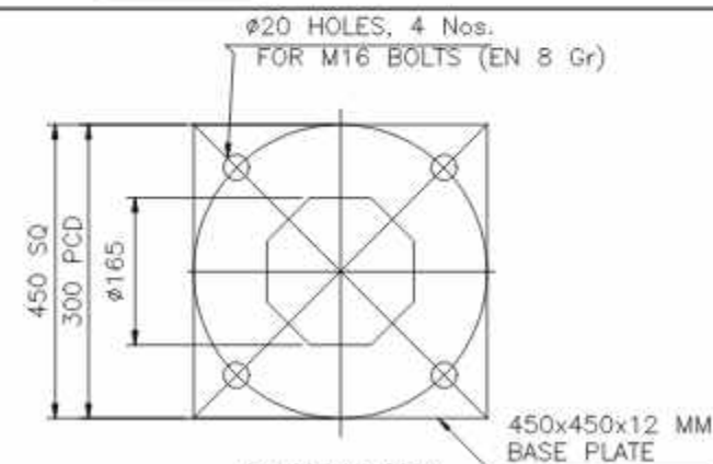
BASE PLATE
