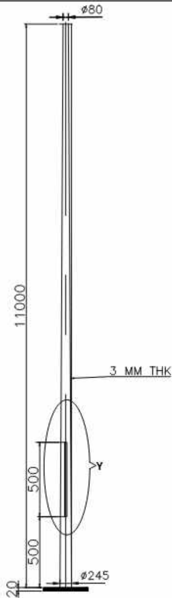
GA. DWG. OF 11 MTR. HEIGHT STANDARD CONICAL POLE
