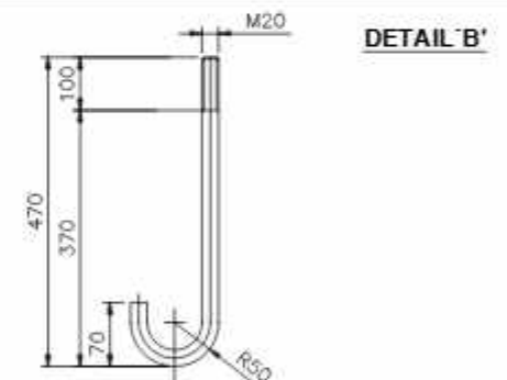
ANCHOR BOLT DETAIL (TOTAL LENGTH-470 mm)
