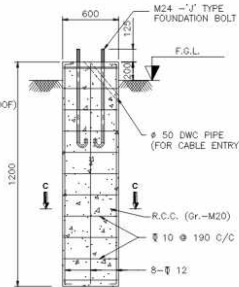
DETAIL OF CIVIL FOUNDATION
