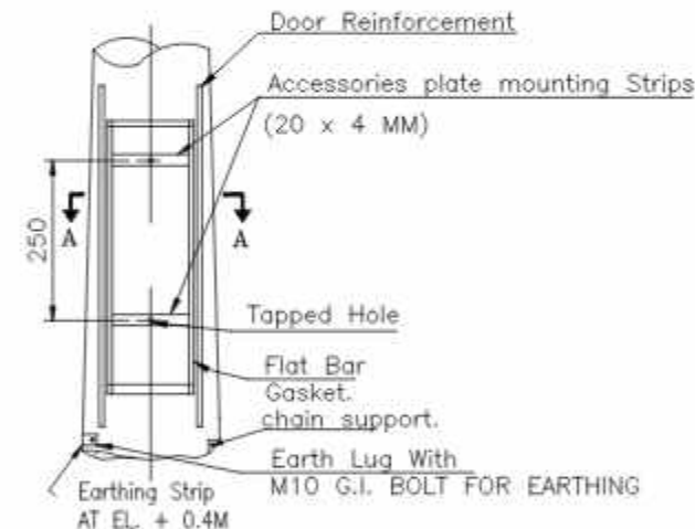
DETAIL 'Y'
