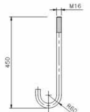
ANCHOR BOLT DETAIL (TOTAL LENGTH=600 mm)
